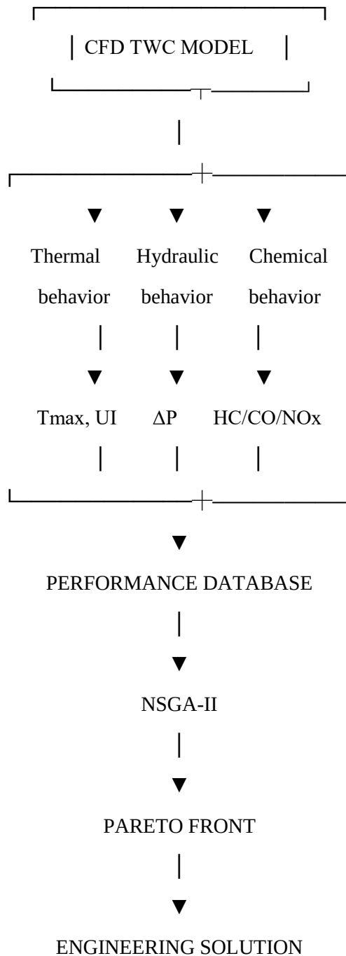
Figure 6. Proposed CFD–NSGA-II optimization framework for the flow-direction-transformed TWC.
